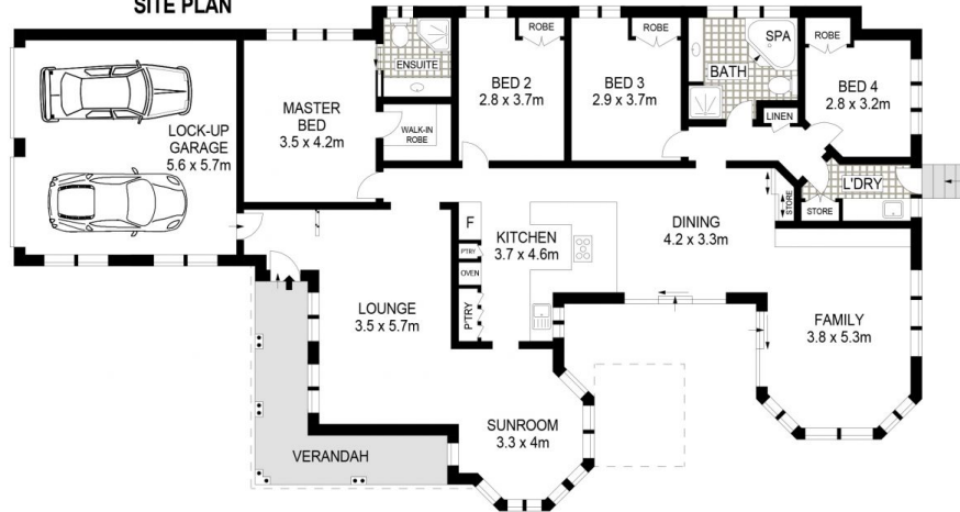
SITE PLAN
