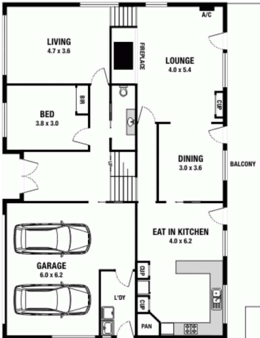
GROUND FLOOR
