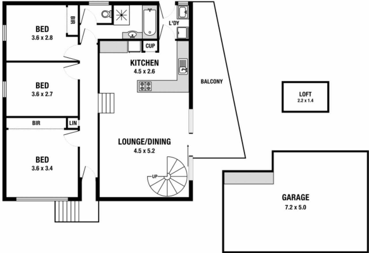
GROUND FLOOR
